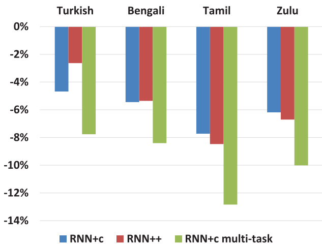
Fig. 8. Relative PPL reduction of RNN+c LMs and RNN++ LMs over RNN LMs for the LLP condition on the test set.
