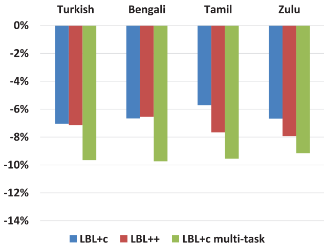
Fig. 7. Relative PPL reduction of LBL+c LMs and LBL++ LMs over LBL LMs for the LLP condition on the test set.
