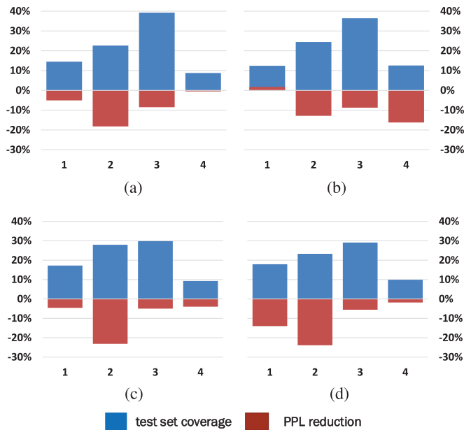
Fig. 11. Relative PPL (on test) reduction of RNN+c LMs using multi-task training over RNN LMs. The X-axis is labelled with the number b , which indicates the number of tokens in test set that occur c \in [10^{b-1}, 10^b) times in the LLP training data. (a) Turkish (b) Bengali (c) Tamil (d) Zulu.
