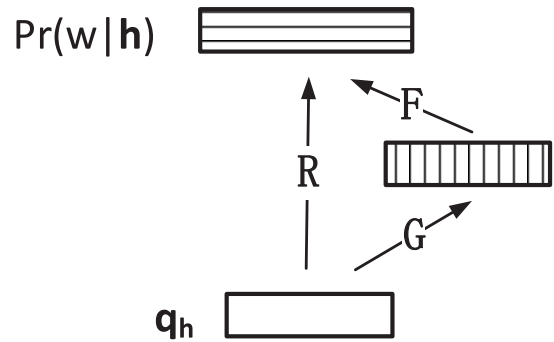
Fig. 5. Additional factor hidden layer between the layer representing \mathbf{q}_h and the output layer. The factor hidden layer is a linear layer with no transformation. It is connected to the softmax output layer with a dictionary-specified weight matrix \mathbf{F} representing the mapping from the word to its morphs.
